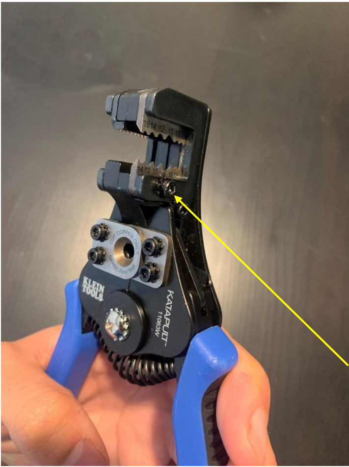
Step 1 Remove the screw indicated.
